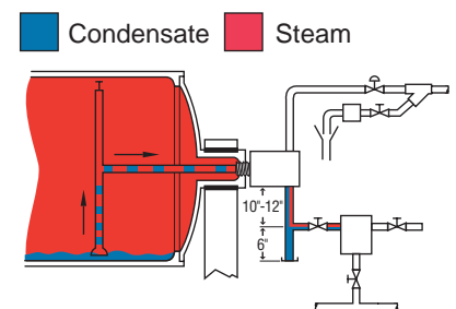
Figure CG-23. Large cylinder, siphon drained. 500 lbs/hr from a 4’ diameter, 10’ long cylinder dryer with 115 cu ft of space at 30 psig. The safety factor is 3:1 with a DC and 8:1 with an IB.
