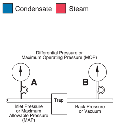
Figure CG-24. "A" minus "B" is Pressure Differential: If "B" is back pressure, subtract it from "A." If "B" is vacuum, add it to "A."
