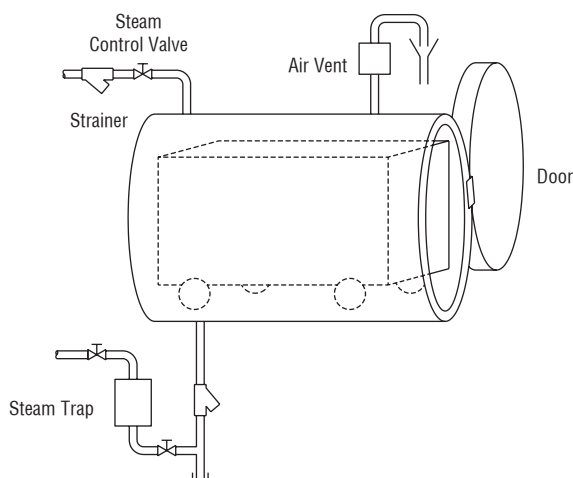
Figure CG-53. Direct Steam Injection Into Product Chamber
