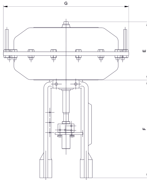
Pneumatic Actuator
