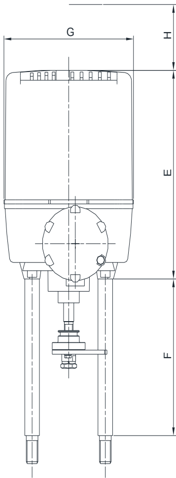
Electric Actuator
