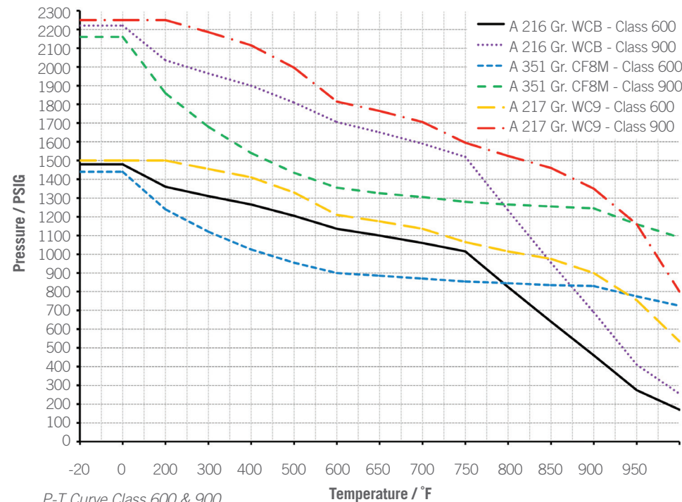
P-T Curve Class 600 & 900
