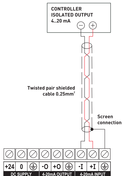
Figure 3.3: Controller with isolated output.
