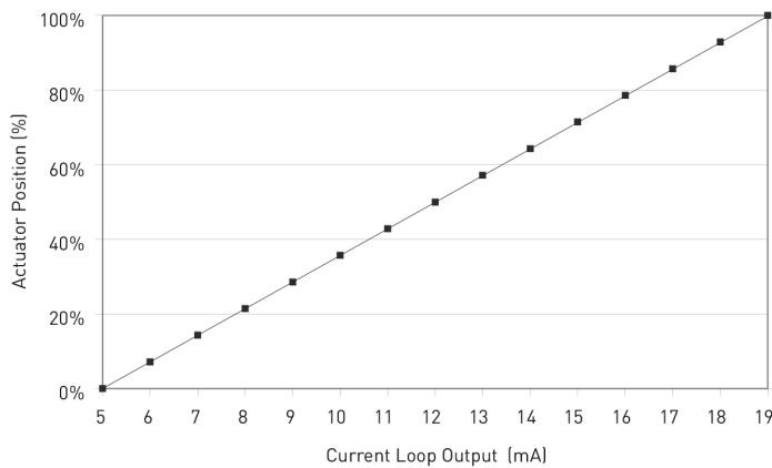
Figure 4.4: Position Control
