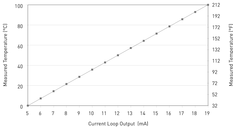
Figure 4.3: Temperature Control
