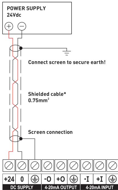
Figure 3.2: Supply Connection
