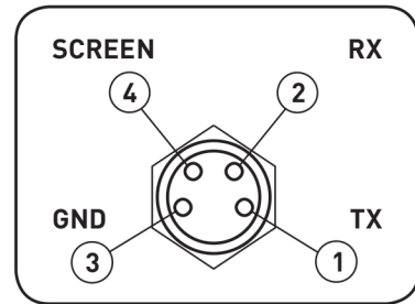
Figure 3.11: RS232 connections on M8 female connector (PORT-2)
