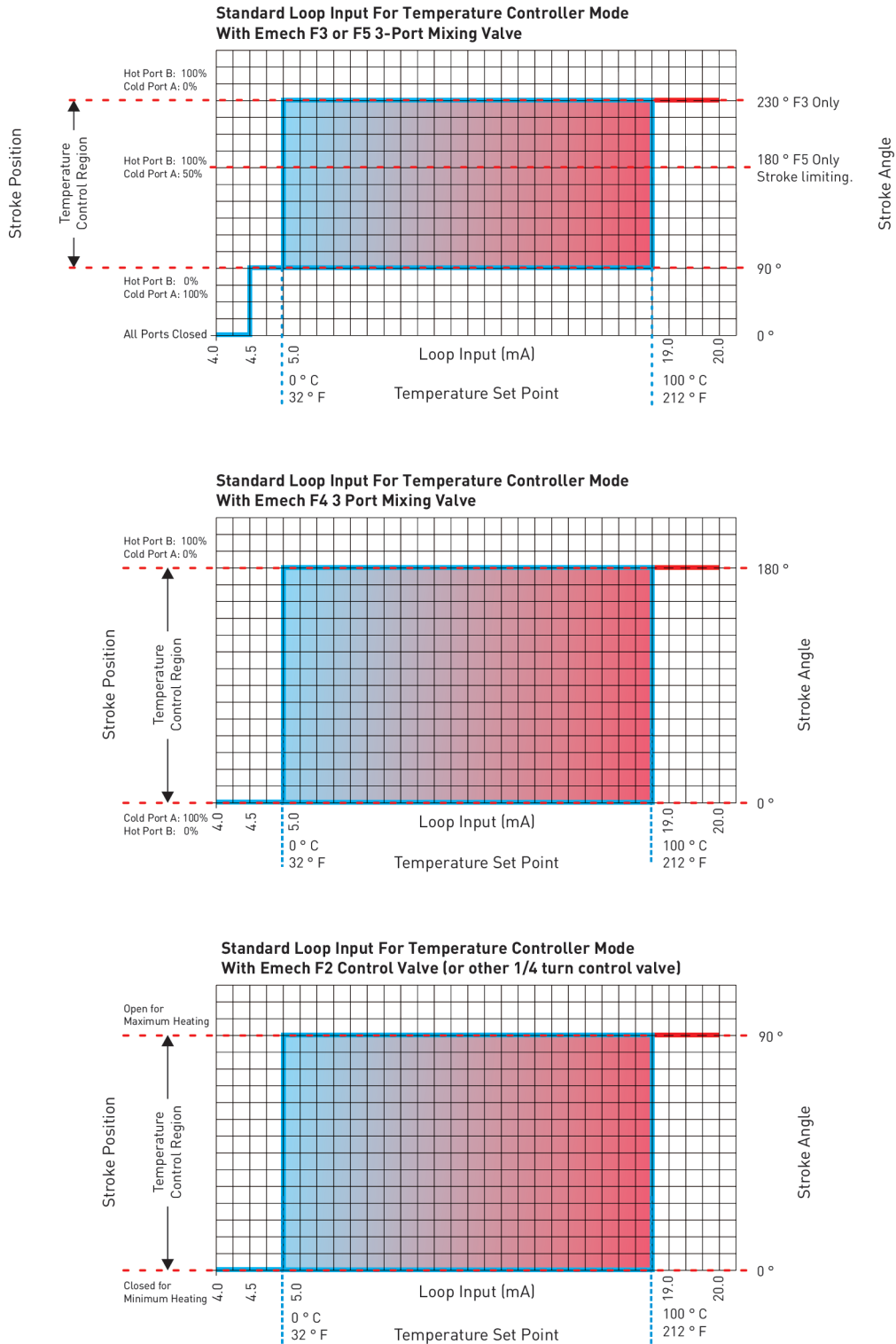
Figure 4.1: Standard Loop Input for Temperature Controller Mode (see page 28).
