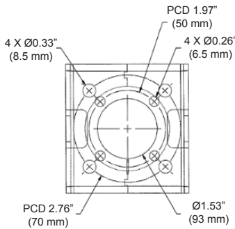
Mounting Bracket Detail (valve side shown)
