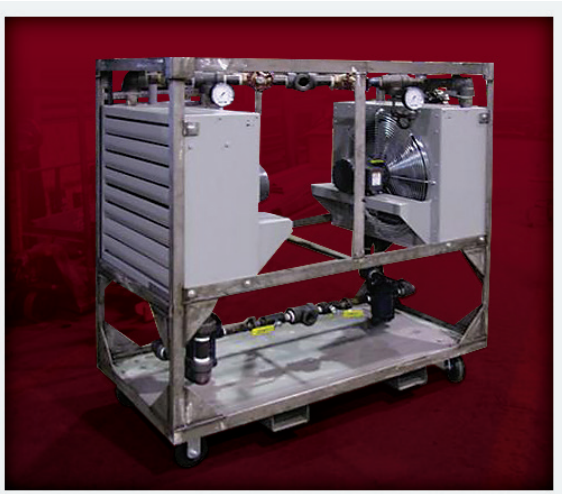
Dual HotBreath Heater for Insect Pest Management
