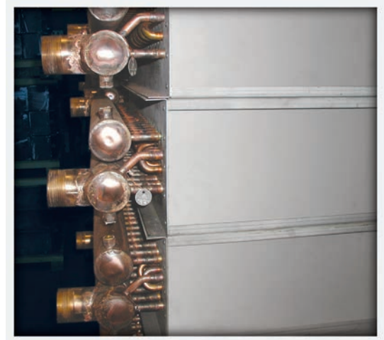
Duralite Plate Fin Coils
