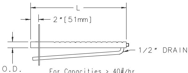
For Capacities > 40#/hr
