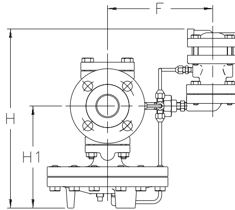
REMOTE MOUNT
