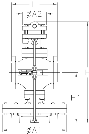
INTEGRAL MOUNT
