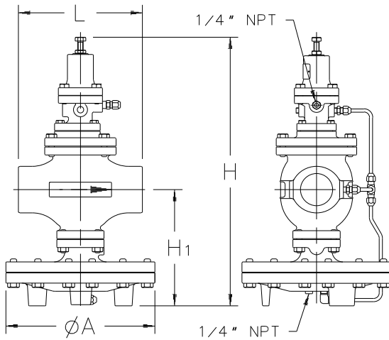
Dimensions & Weights
