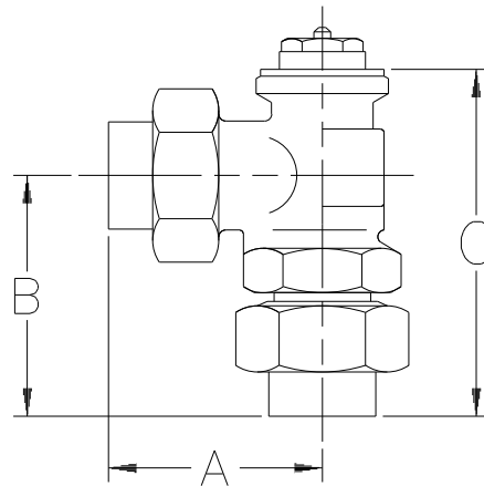
RV-4 ANGLE SOLDER
